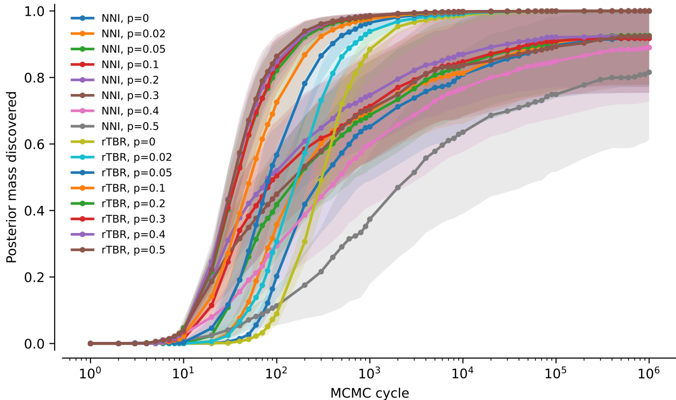
tw5: NNI vs rTBR averaged over alignments: Posterior mass discovered
