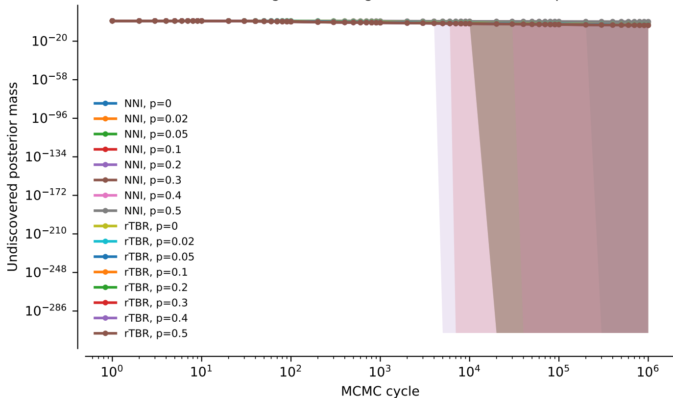
tw5: NNI vs rTBR averaged over alignments: Undiscovered posterior mass
