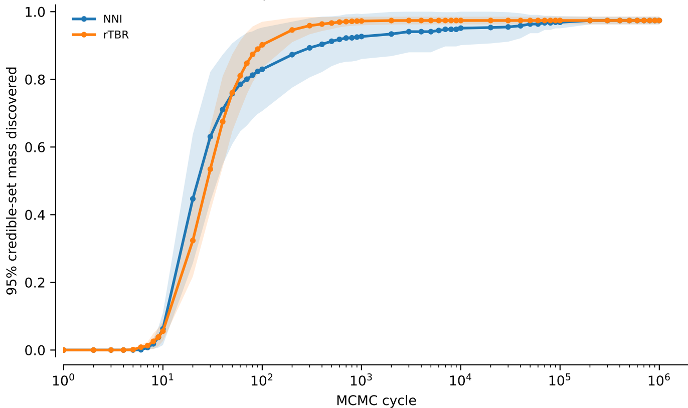
tw0: NNI vs rTBR, power=0.1: 95% credible-set mass discovered
