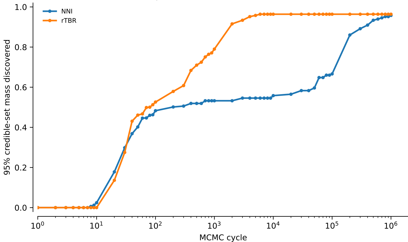
tw2: NNI vs rTBR, power=0.1: 95% credible-set mass discovered
