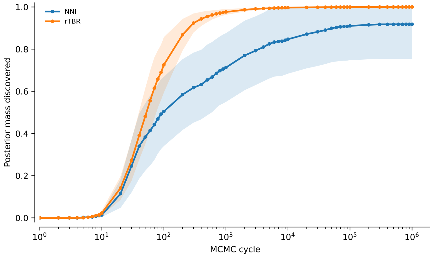
tw5: NNI vs rTBR, power=0.1: Posterior mass discovered
