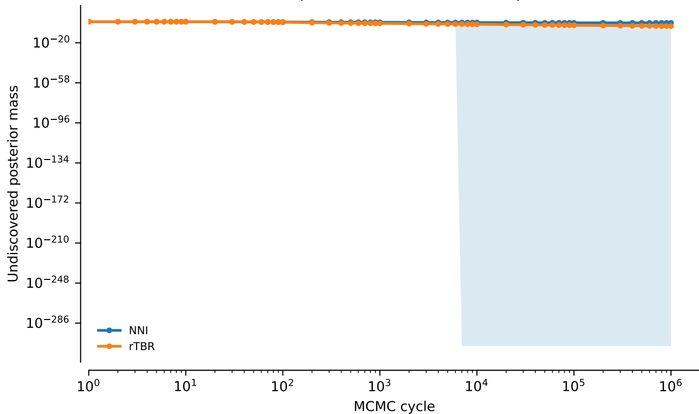
tw5: NNI vs rTBR, power=0.1: Undiscovered posterior mass
