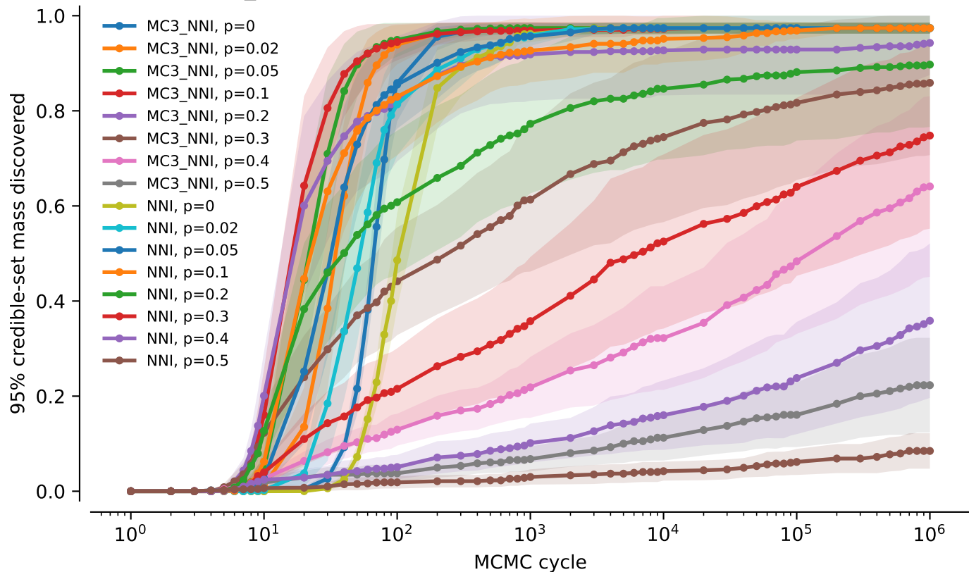
tw0: NNI vs MC3_NNI averaged over alignments: 95% credible-set mass discovered
