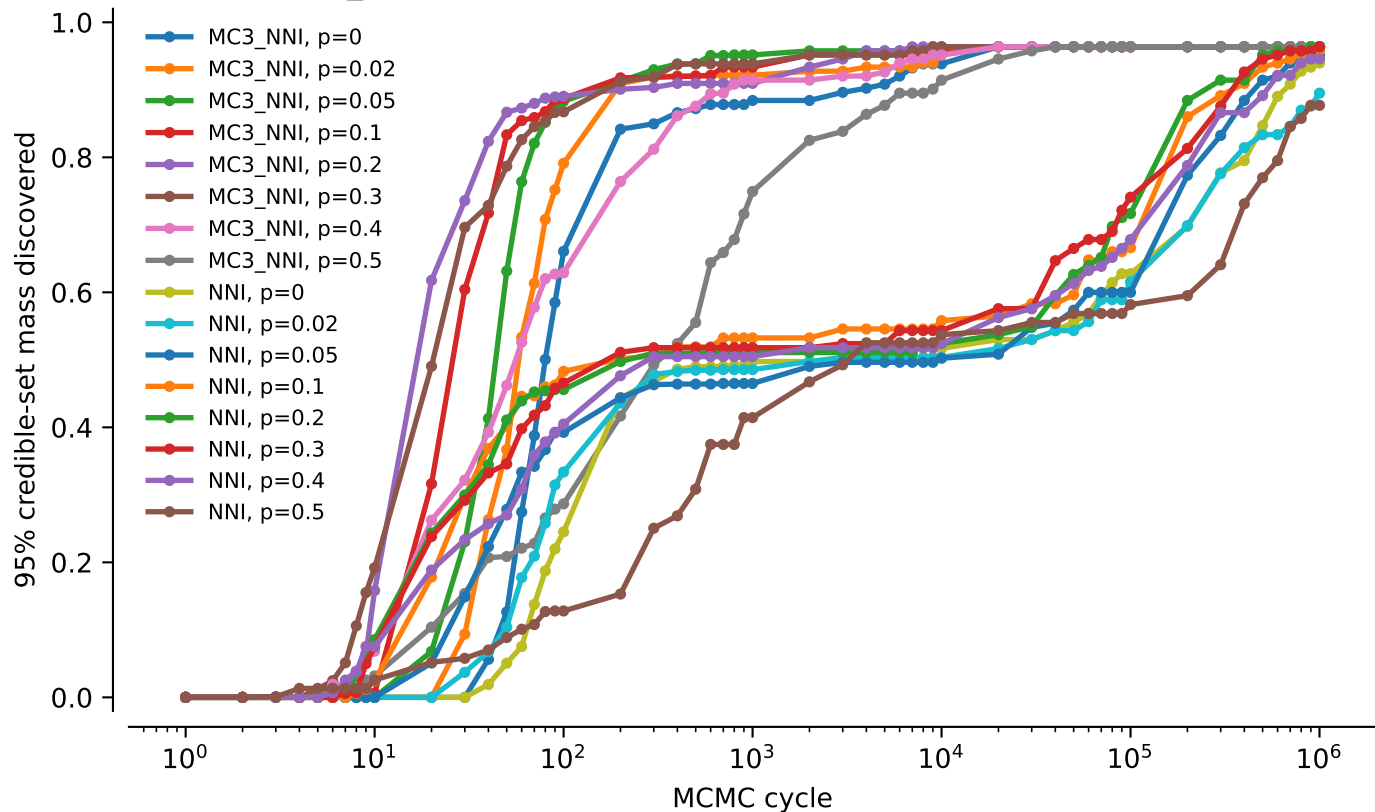
tw2: NNI vs MC3_NNI averaged over alignments: 95% credible-set mass discovered
