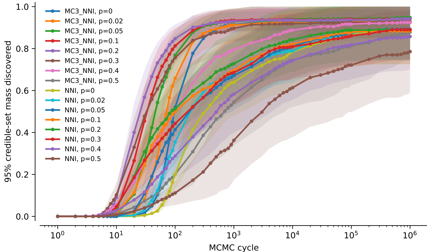
tw5: NNI vs MC3_NNI averaged over alignments: 95% credible-set mass discovered
