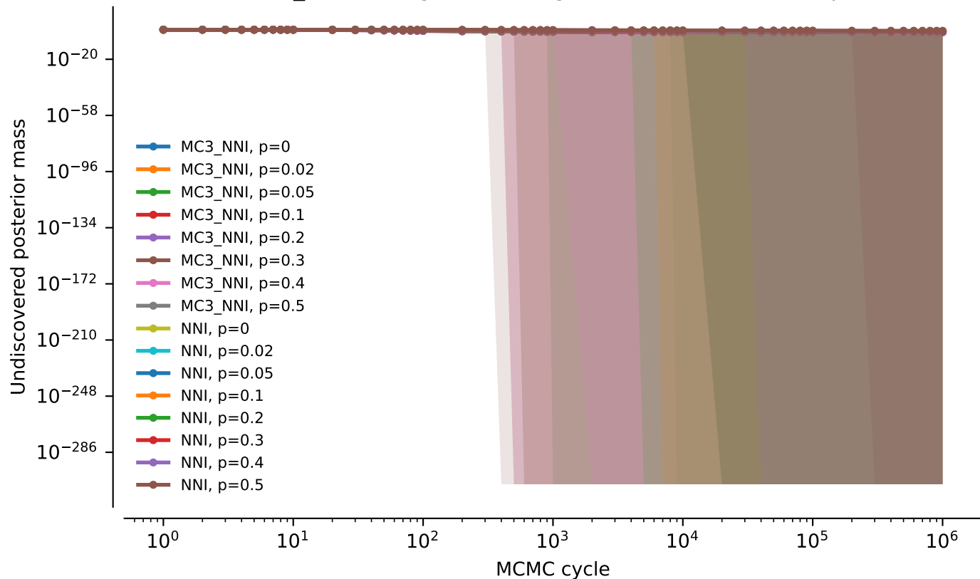
tw5: NNI vs MC3_NNI averaged over alignments: Undiscovered posterior mass
