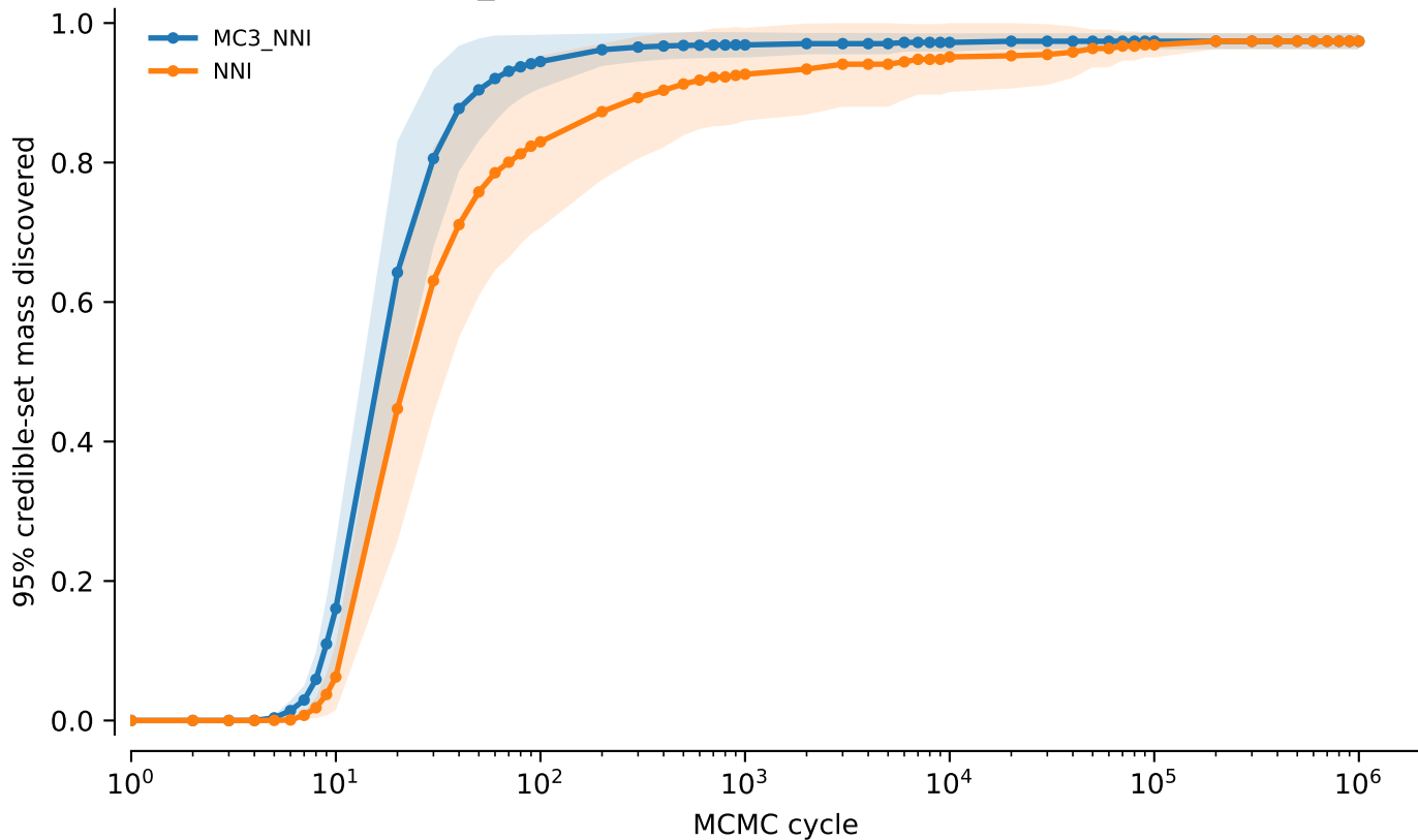
tw0: NNI vs MC3_NNI, power=0.1: 95% credible-set mass discovered
