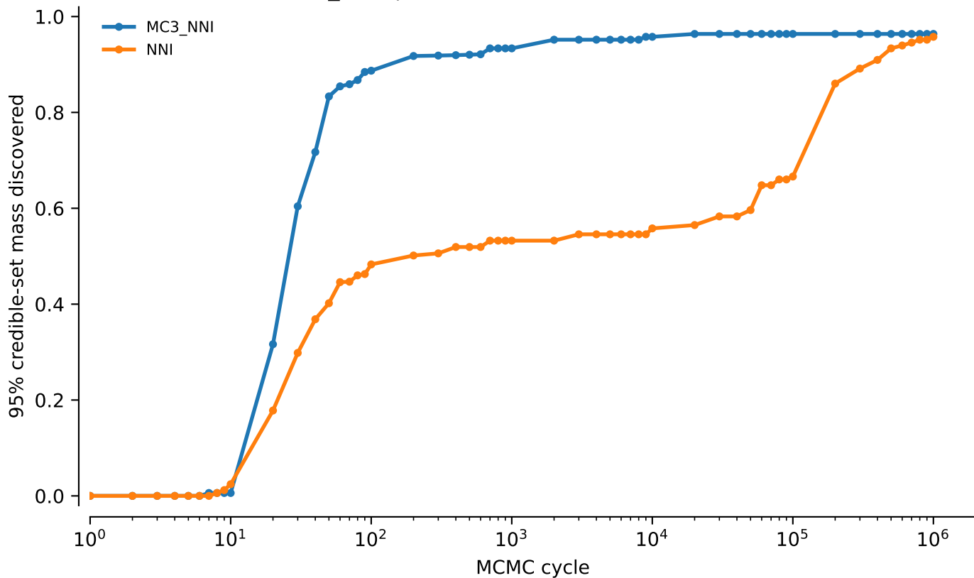
tw2: NNI vs MC3_NNI, power=0.1: 95% credible-set mass discovered
