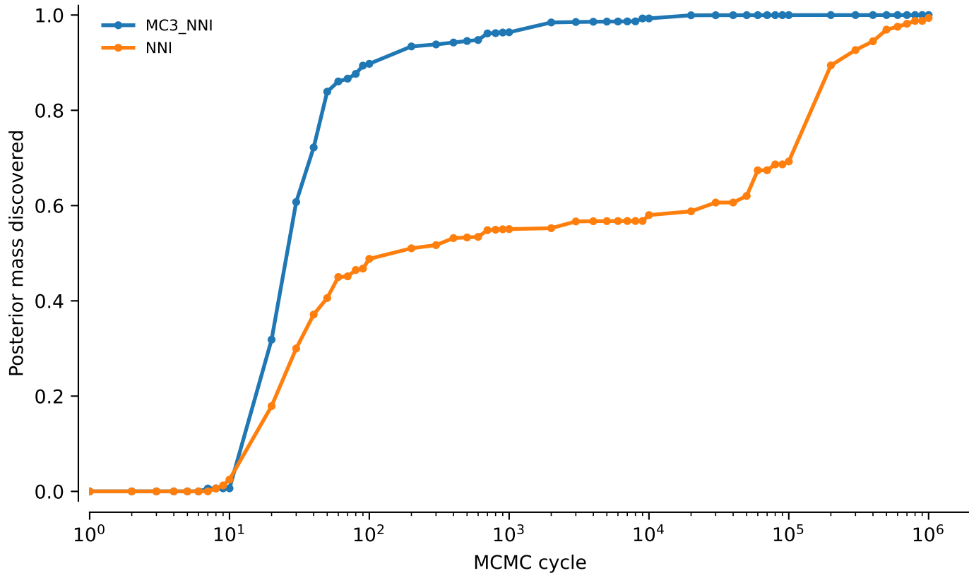
tw2: NNI vs MC3_NNI, power=0.1: Posterior mass discovered
