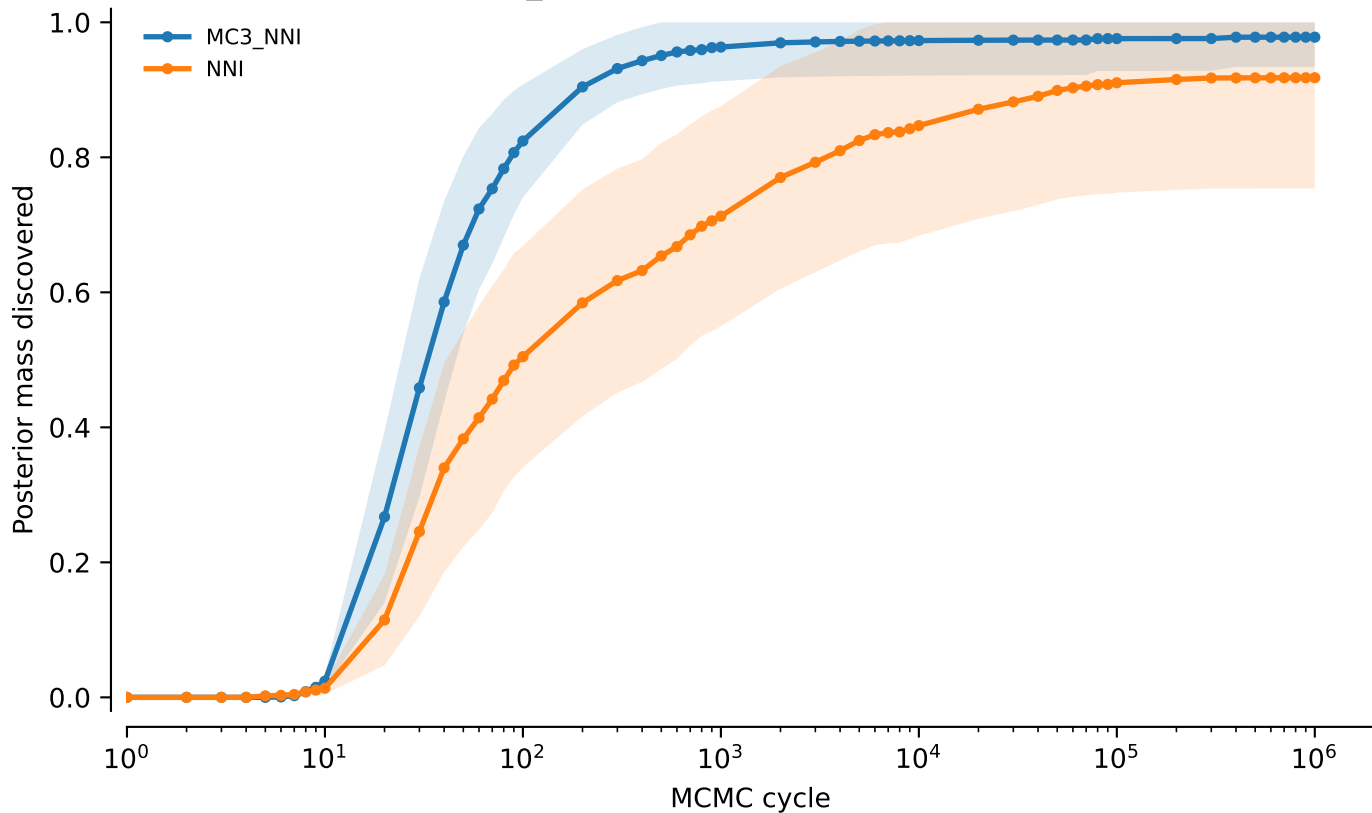
tw5: NNI vs MC3_NNI, power=0.1: Posterior mass discovered
