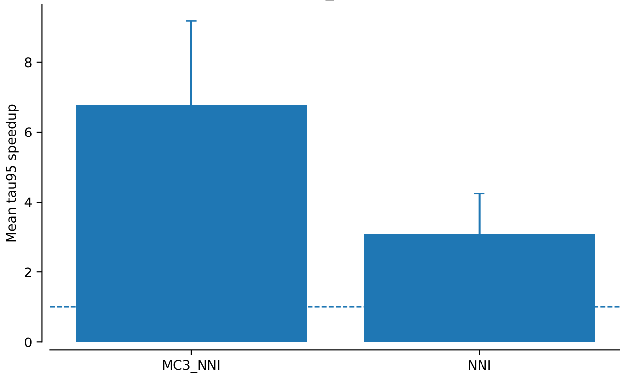
tw0: NNI vs MC3_NNI at power=0.1
