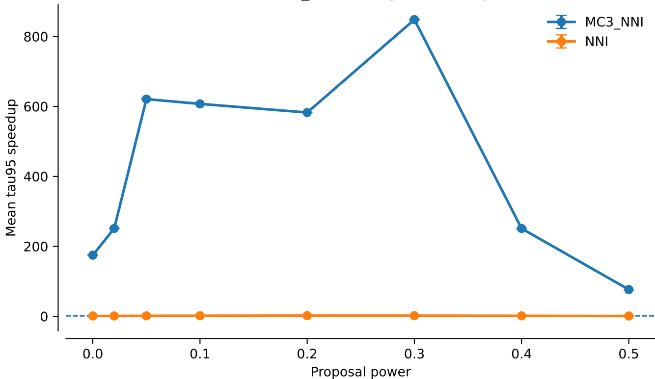
tw2: NNI vs MC3_NNI averaged over alignments
