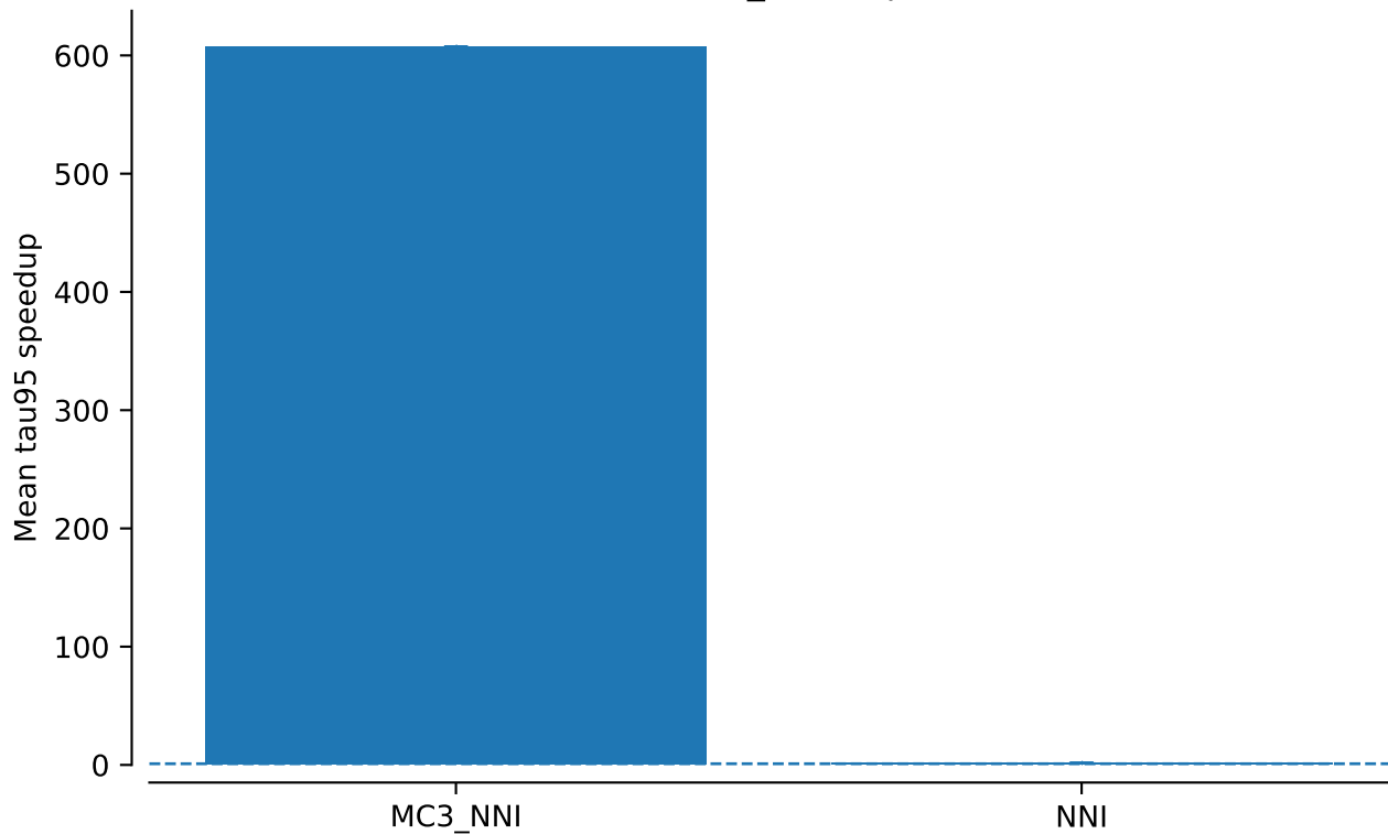
tw2: NNI vs MC3_NNI at power=0.1
