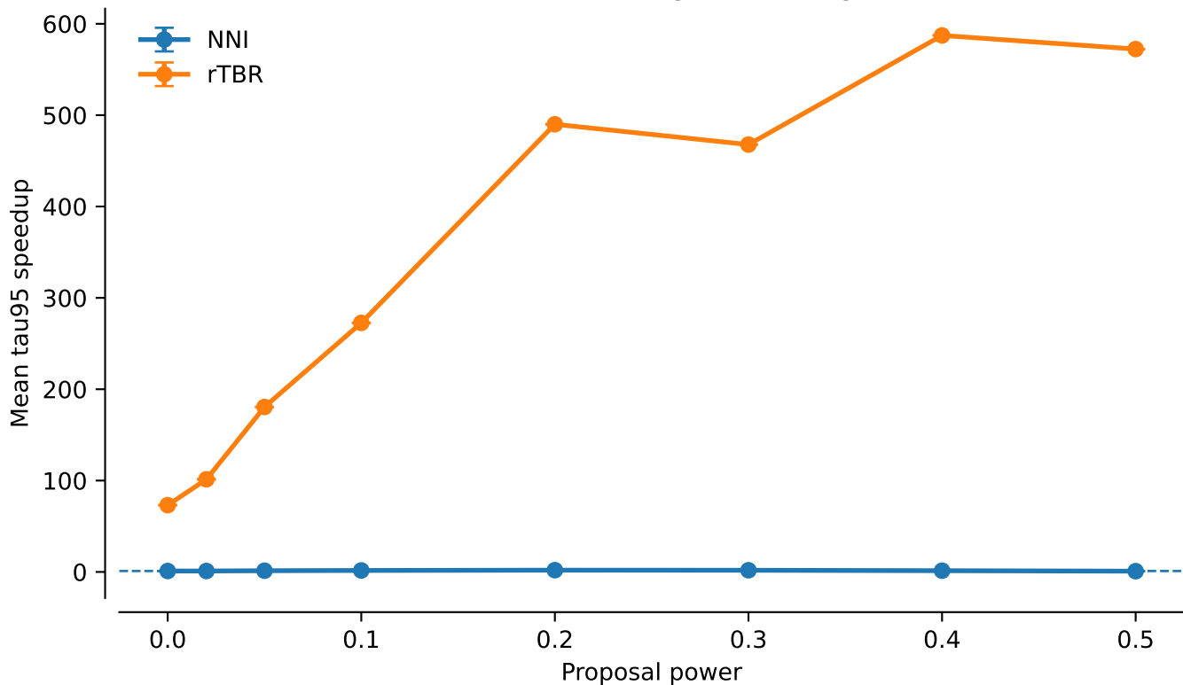
tw2: NNI vs rTBR averaged over alignments
