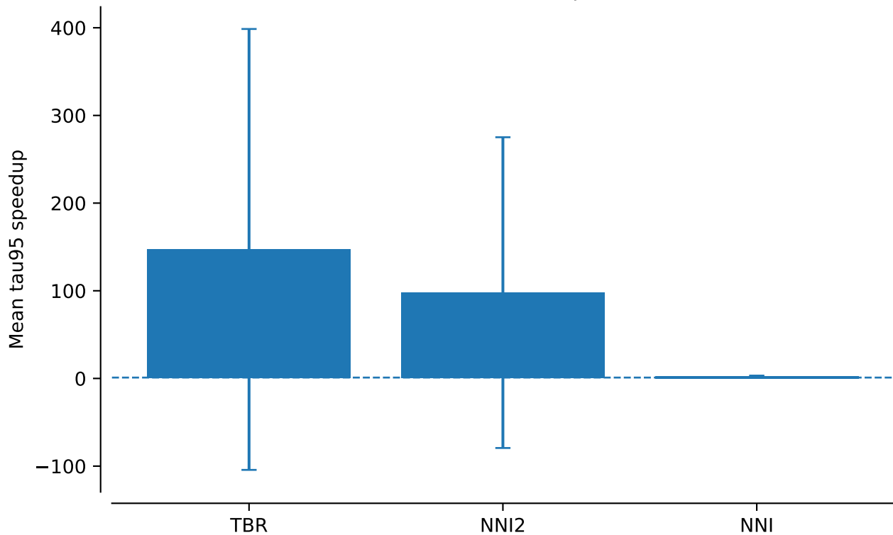
tw5: NNI, NNI2, TBR at power=0.1
