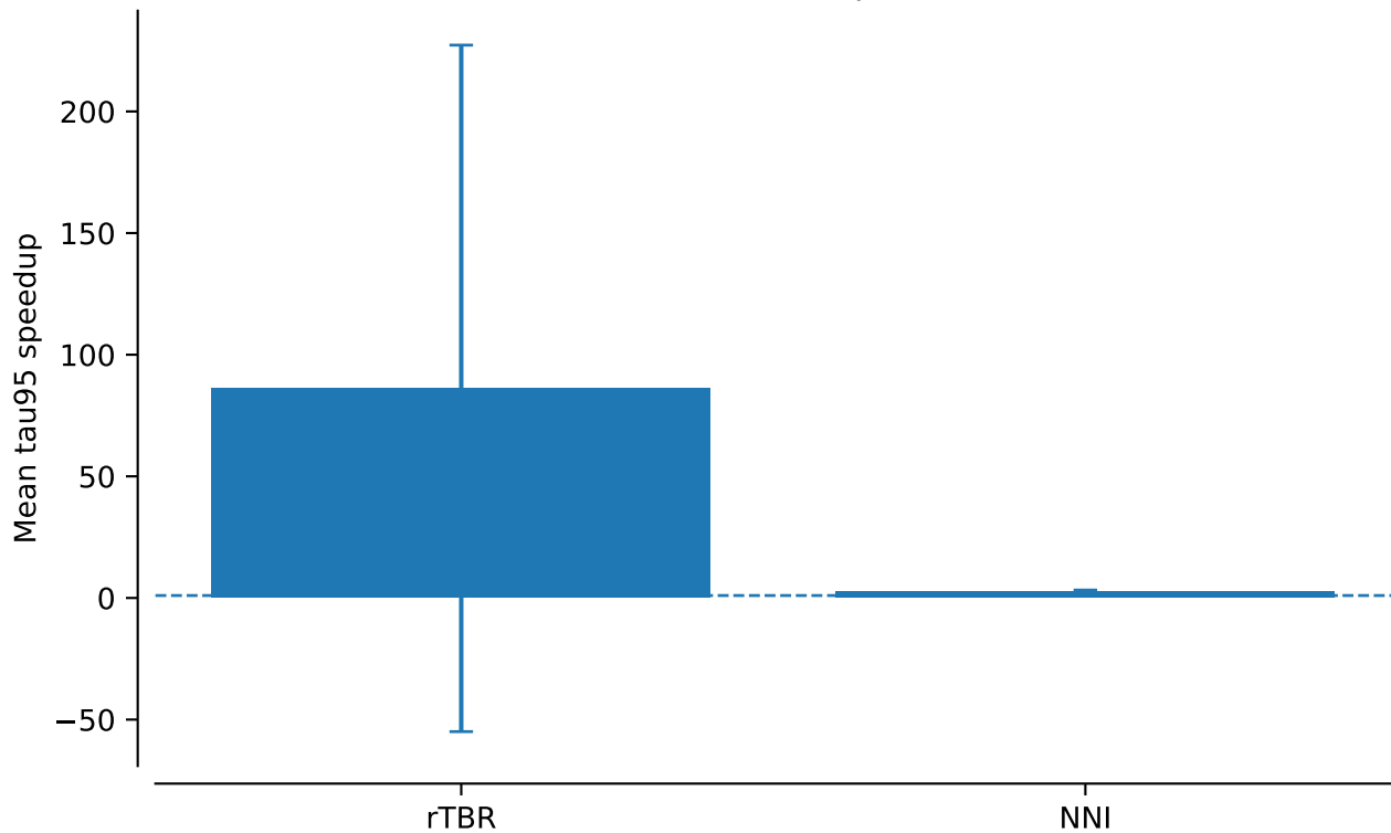
tw5: NNI vs rTBR at power=0.1
