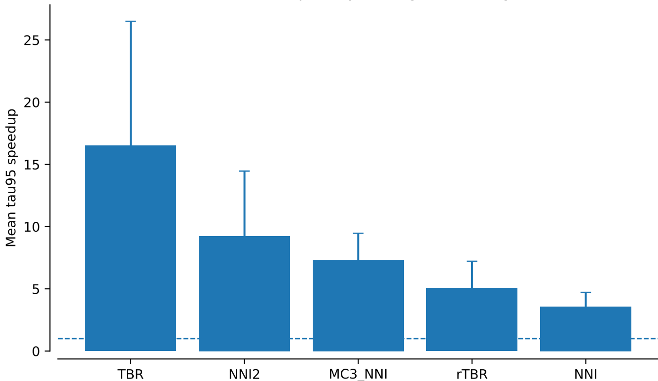
tw0: best method speedup averaged over alignments
