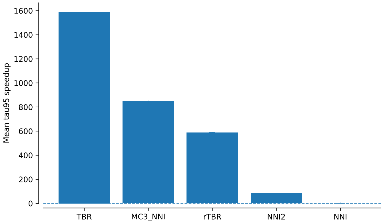
tw2: best method speedup averaged over alignments
