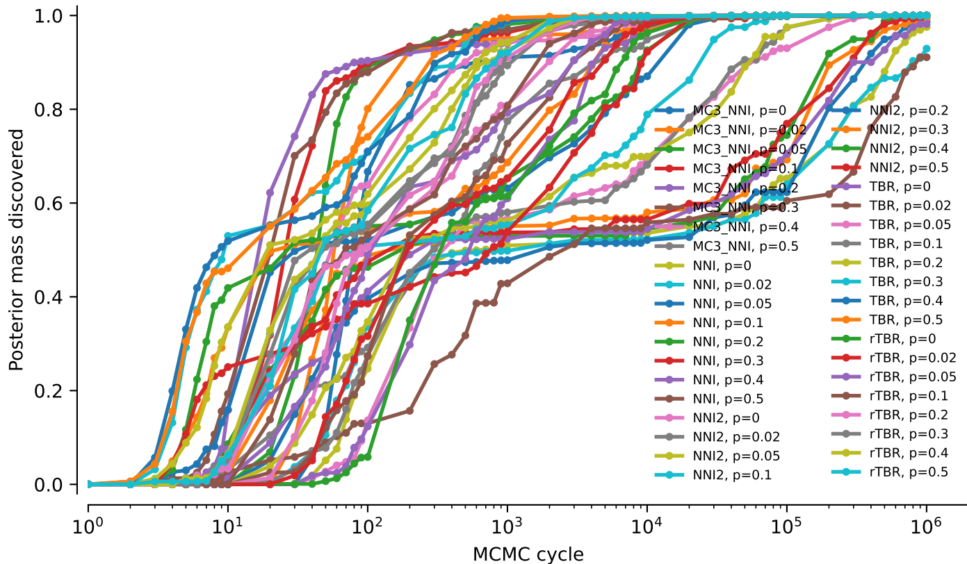
tw2: average over alignments — Posterior mass discovered
