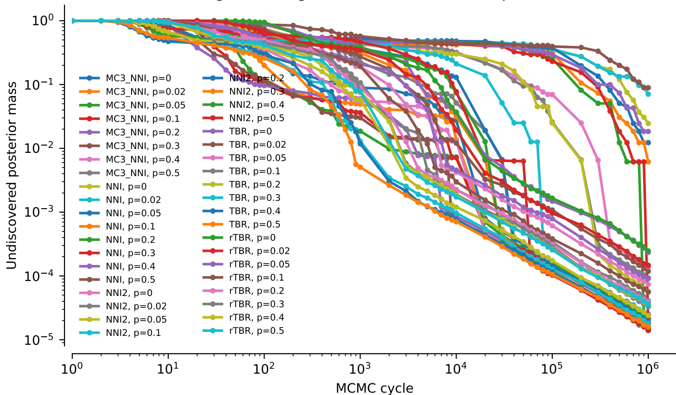
tw2: average over alignments — Undiscovered posterior mass
