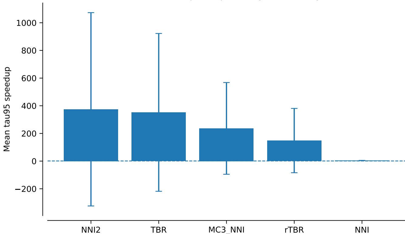
tw5: best method speedup averaged over alignments
