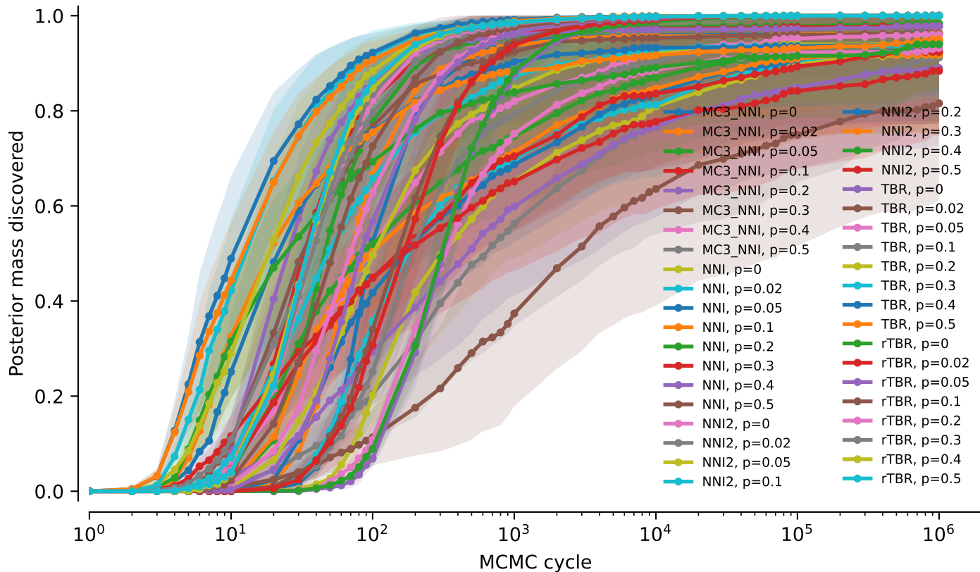
tw5: average over alignments — Posterior mass discovered
