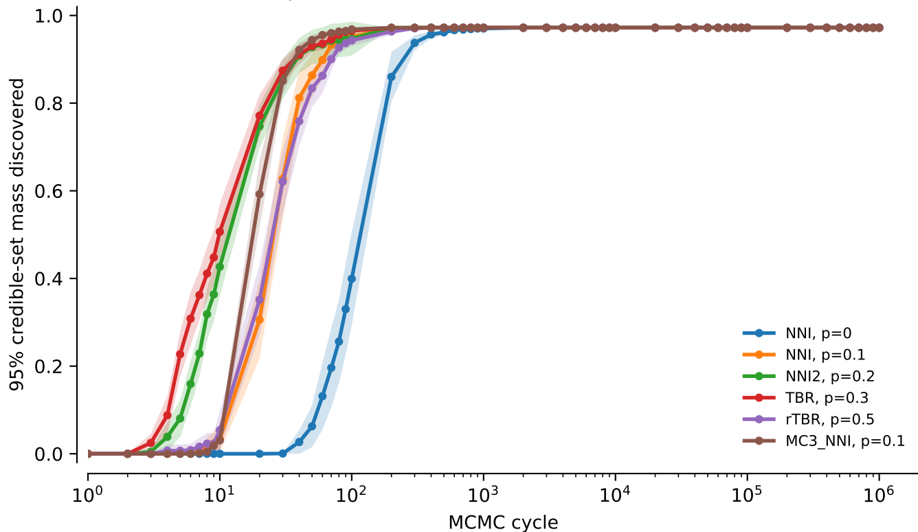
vert.atpase6.tw5: 95% credible-set mass discovered
