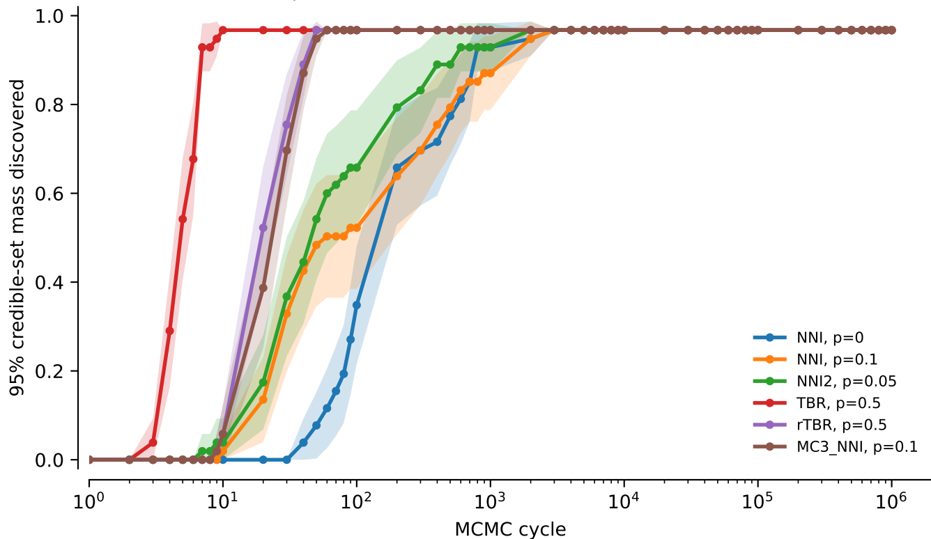
vert.atpase8.tw0: 95% credible-set mass discovered
