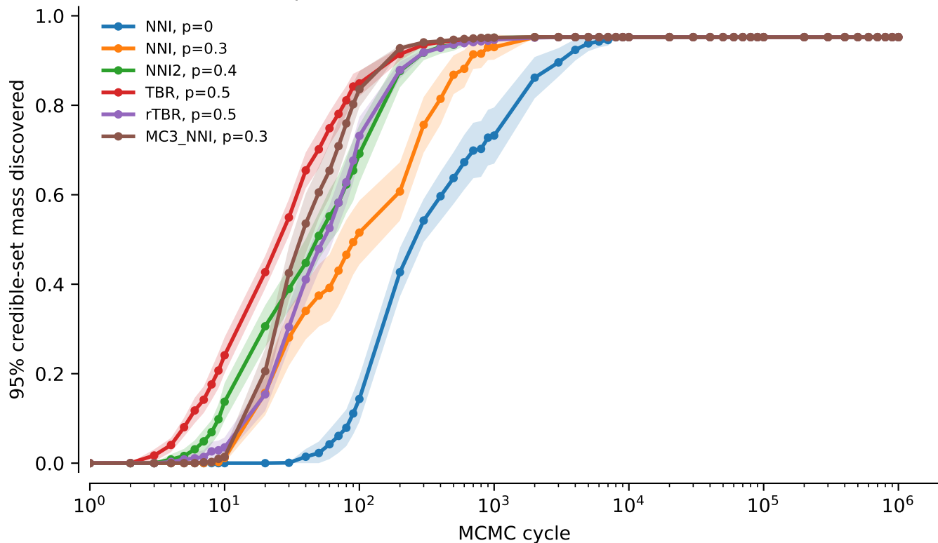
vert.atpase8.tw5: 95% credible-set mass discovered
