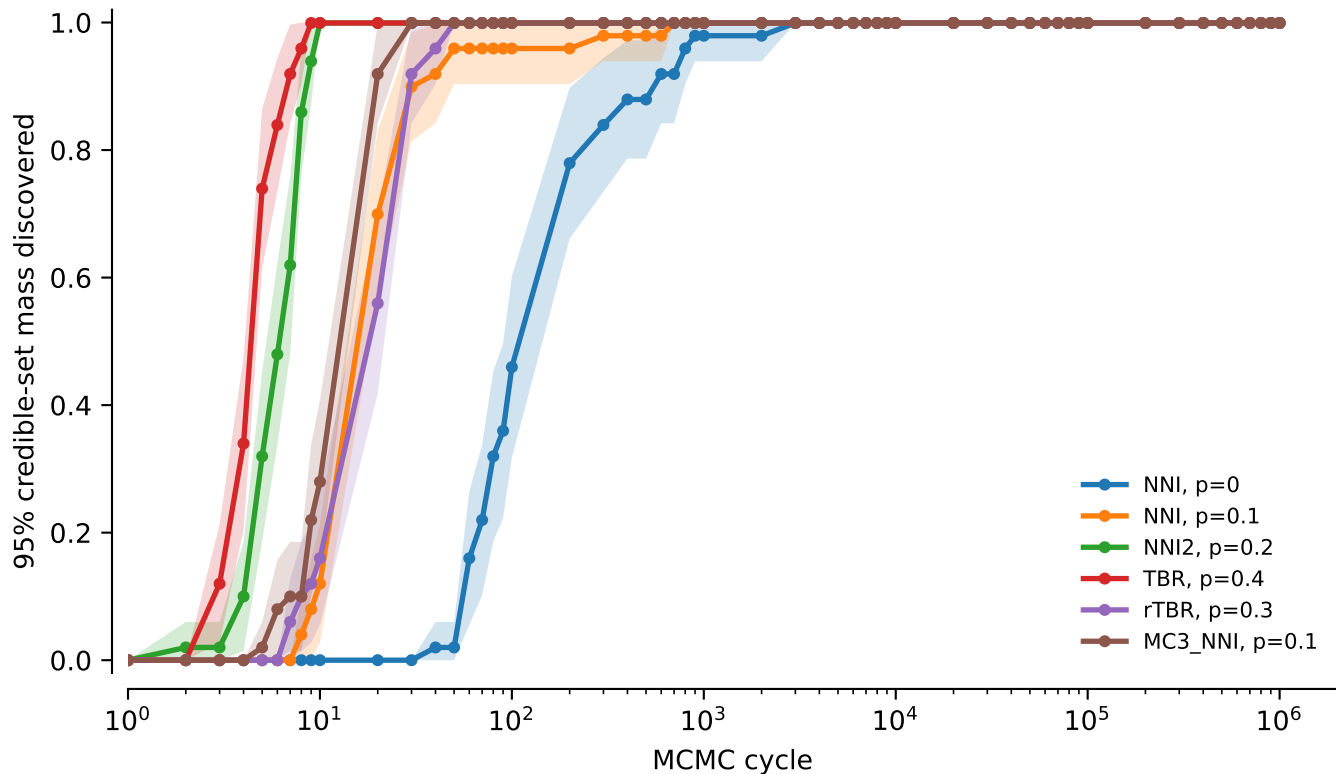
vert.coi.tw0: 95% credible-set mass discovered
