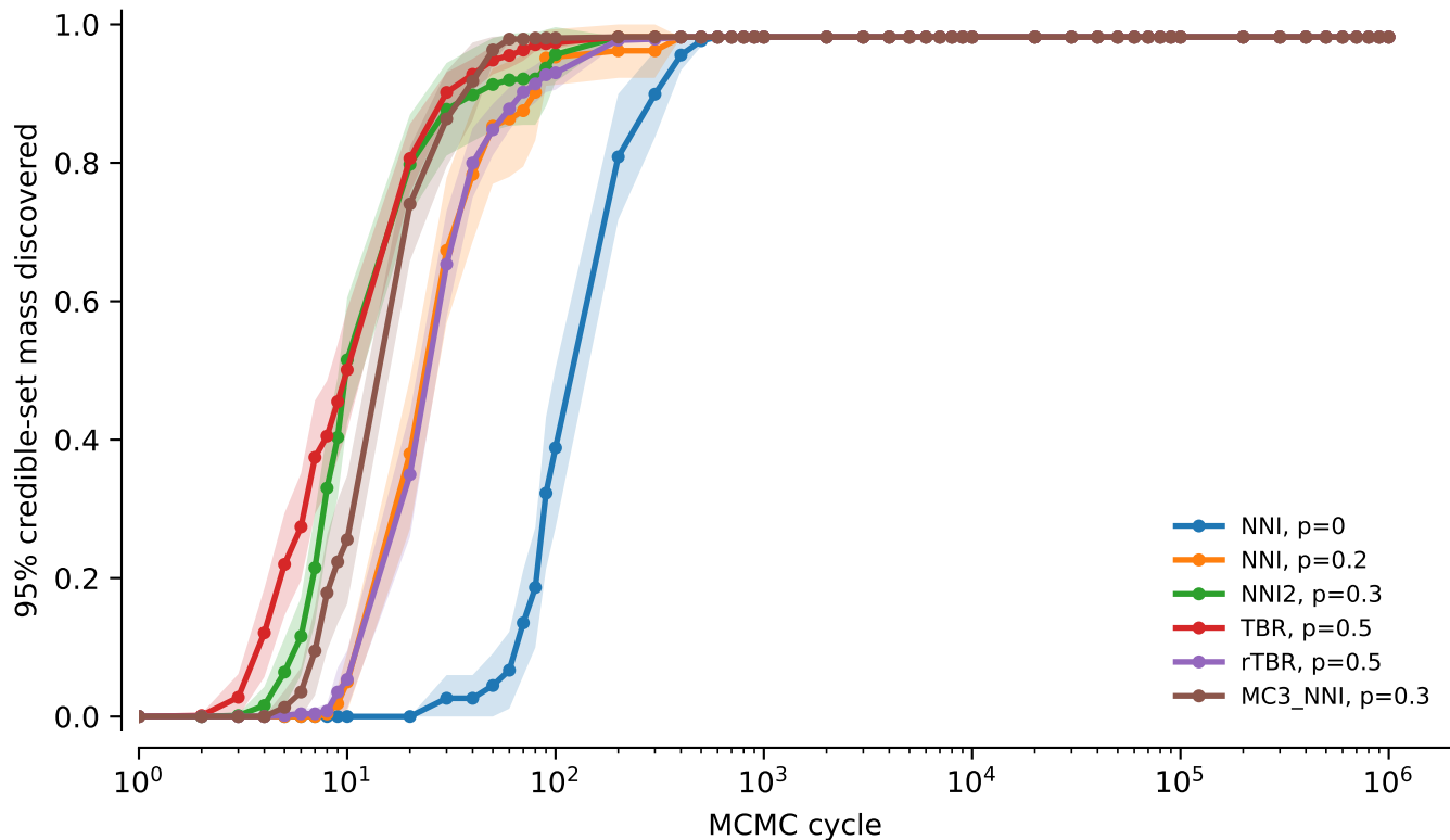
vert.coii.tw5: 95% credible-set mass discovered
