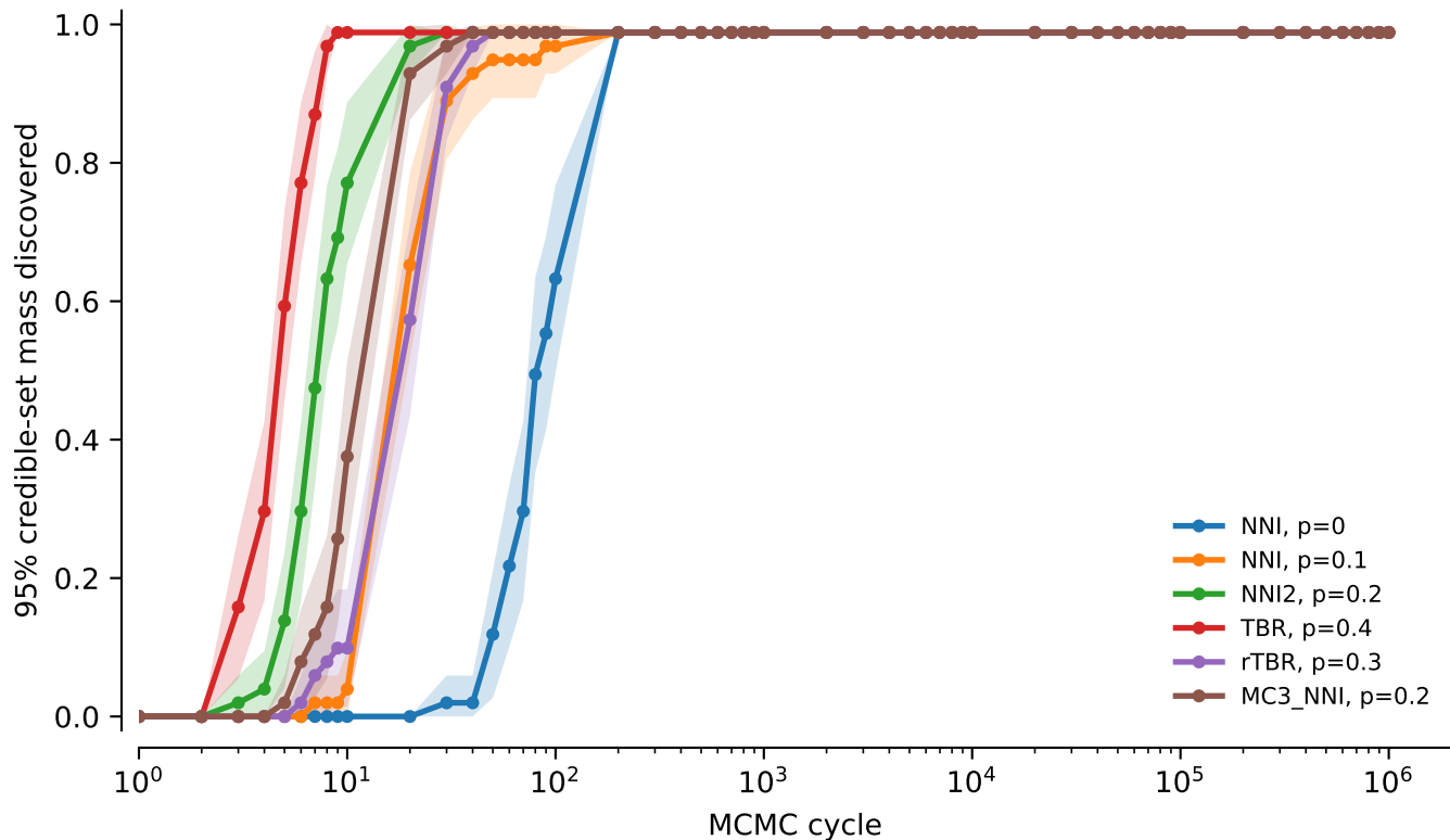
vert.coiii.tw0: 95% credible-set mass discovered
