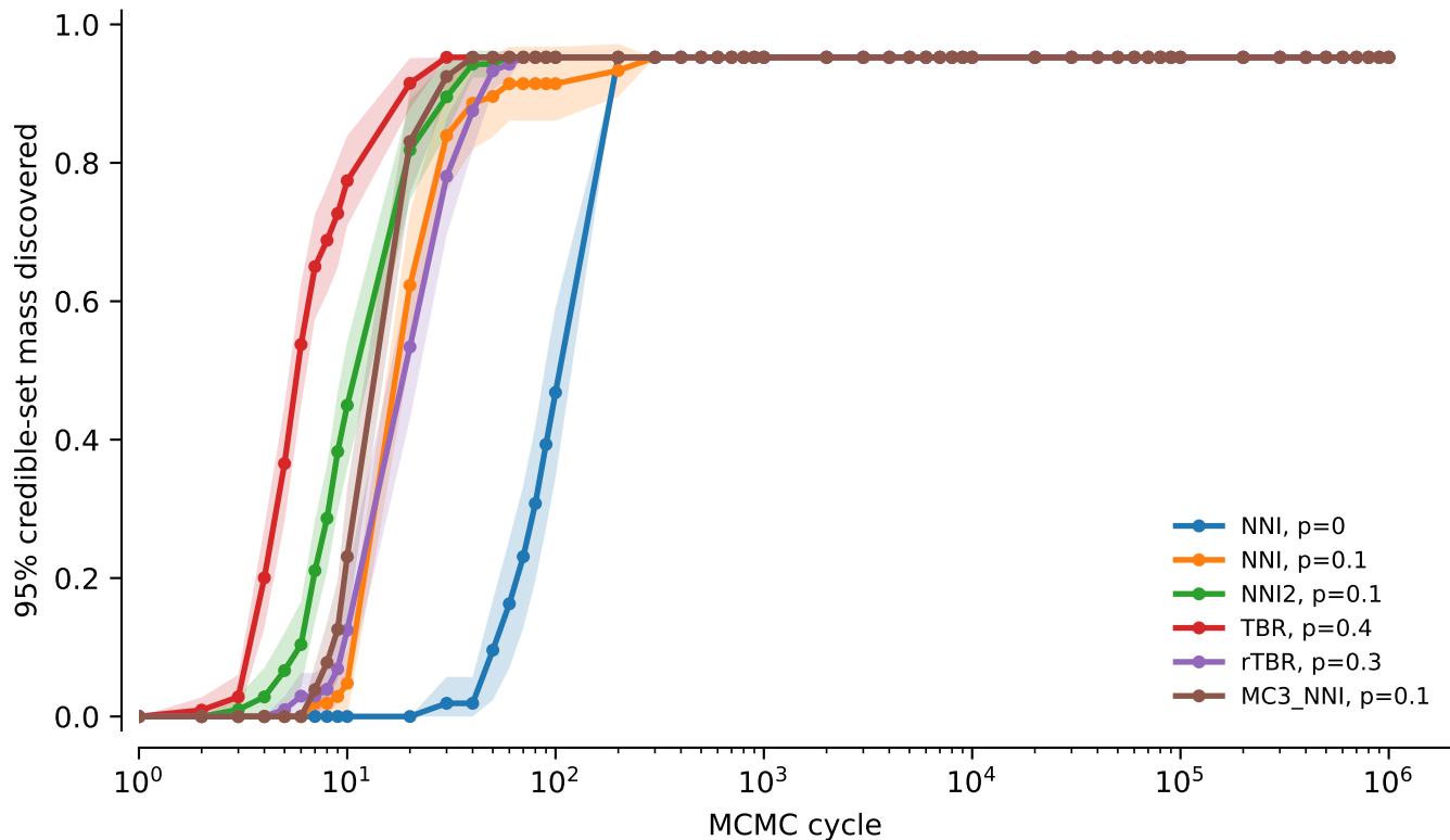
vert.nd1.tw0: 95% credible-set mass discovered
