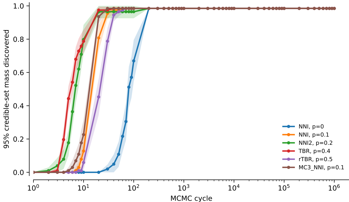
vert.nd2.tw0: 95% credible-set mass discovered
