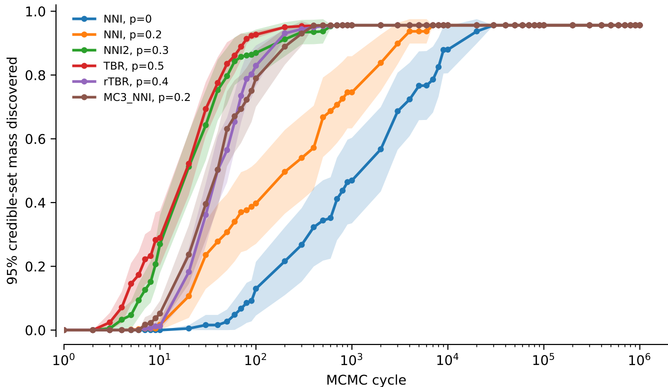
vert.nd2.tw5: 95% credible-set mass discovered
