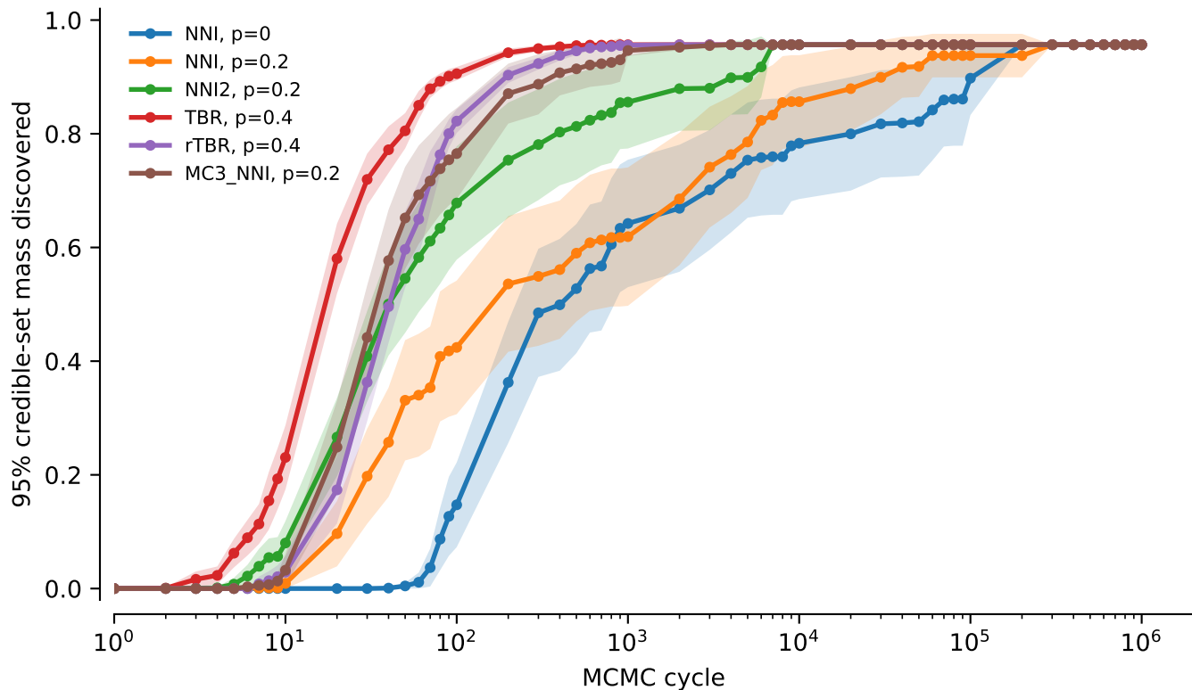
vert.nd3.tw5: 95% credible-set mass discovered
