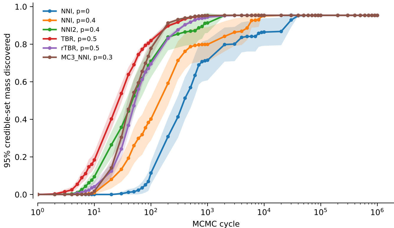
vert.nd4l.tw5: 95% credible-set mass discovered
