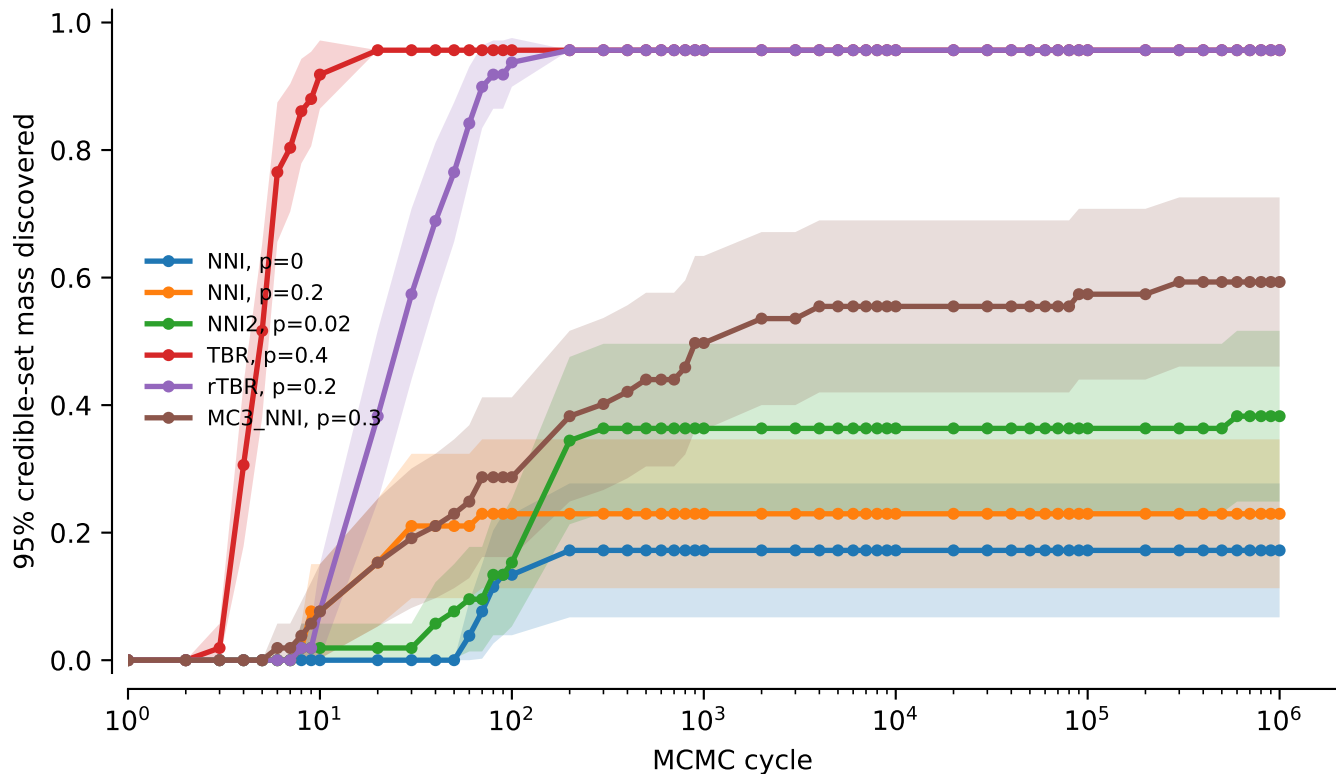
vert.nd6.tw5: 95% credible-set mass discovered
