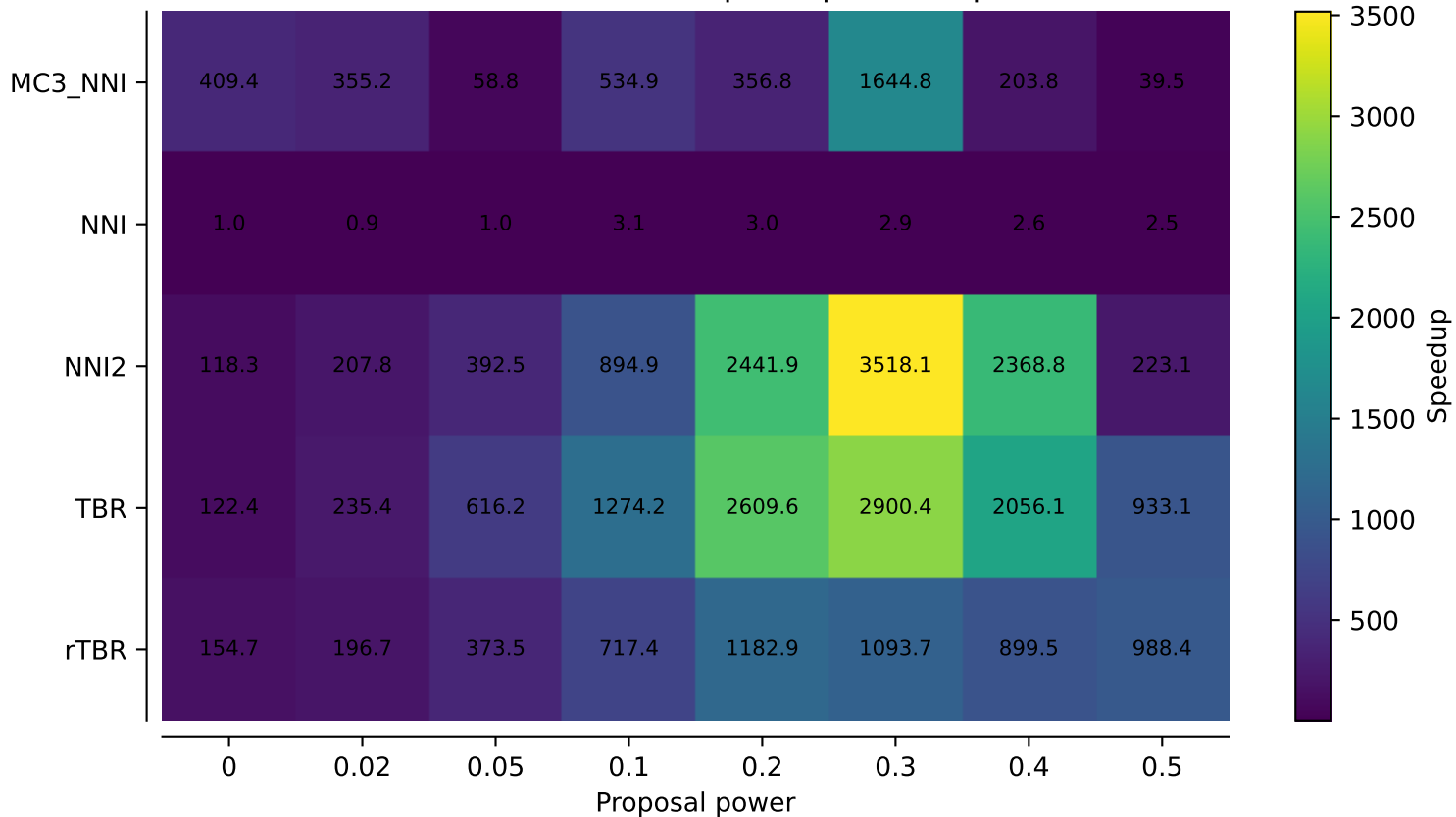
vert.coi.tw5: tau95 speedup heatmap
