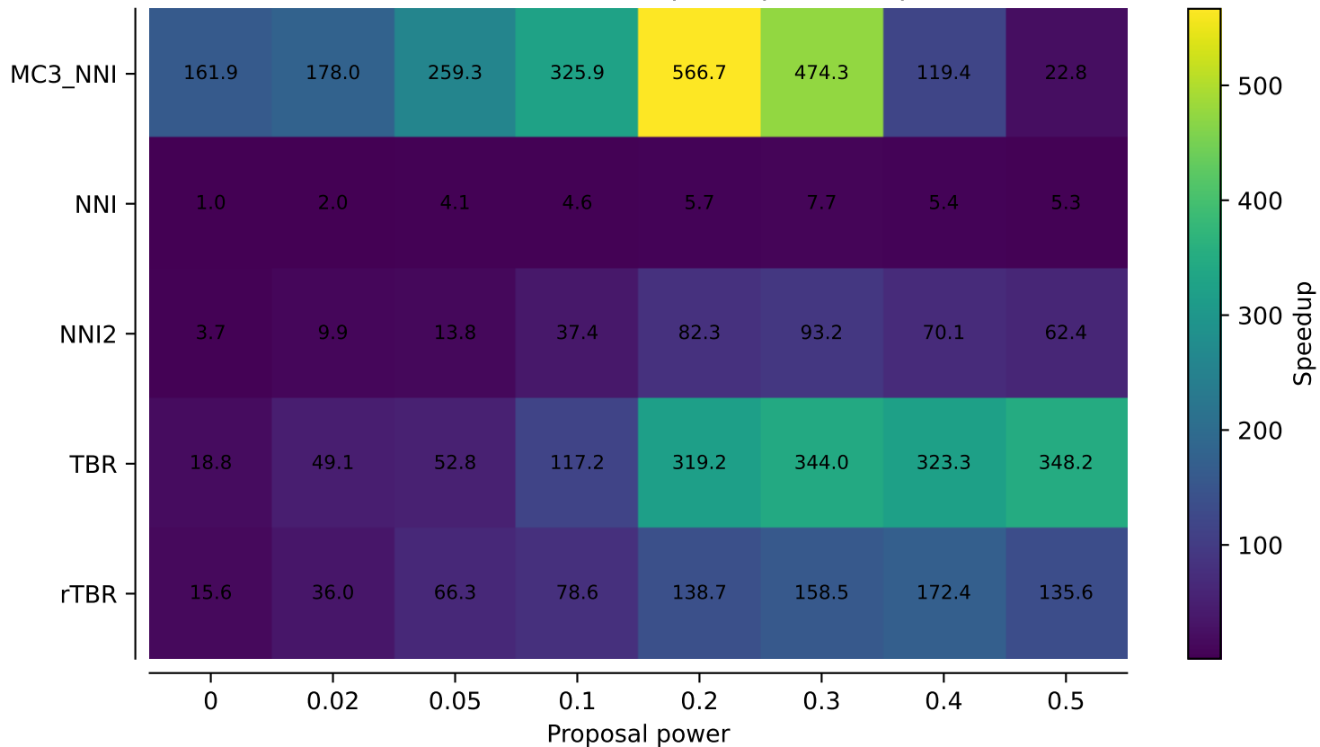
vert.nd1.tw5: tau95 speedup heatmap
