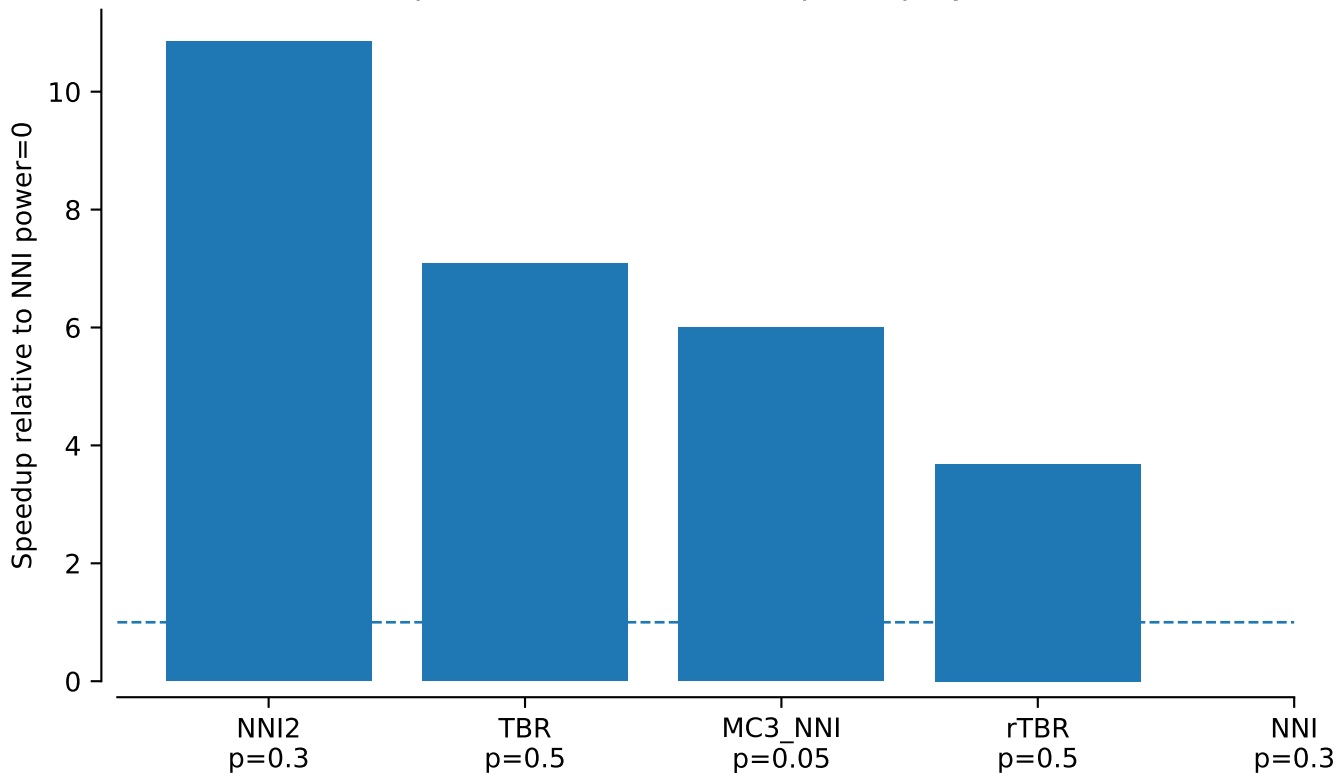
vert.atpase6.tw0: best tau95 speedup by method
