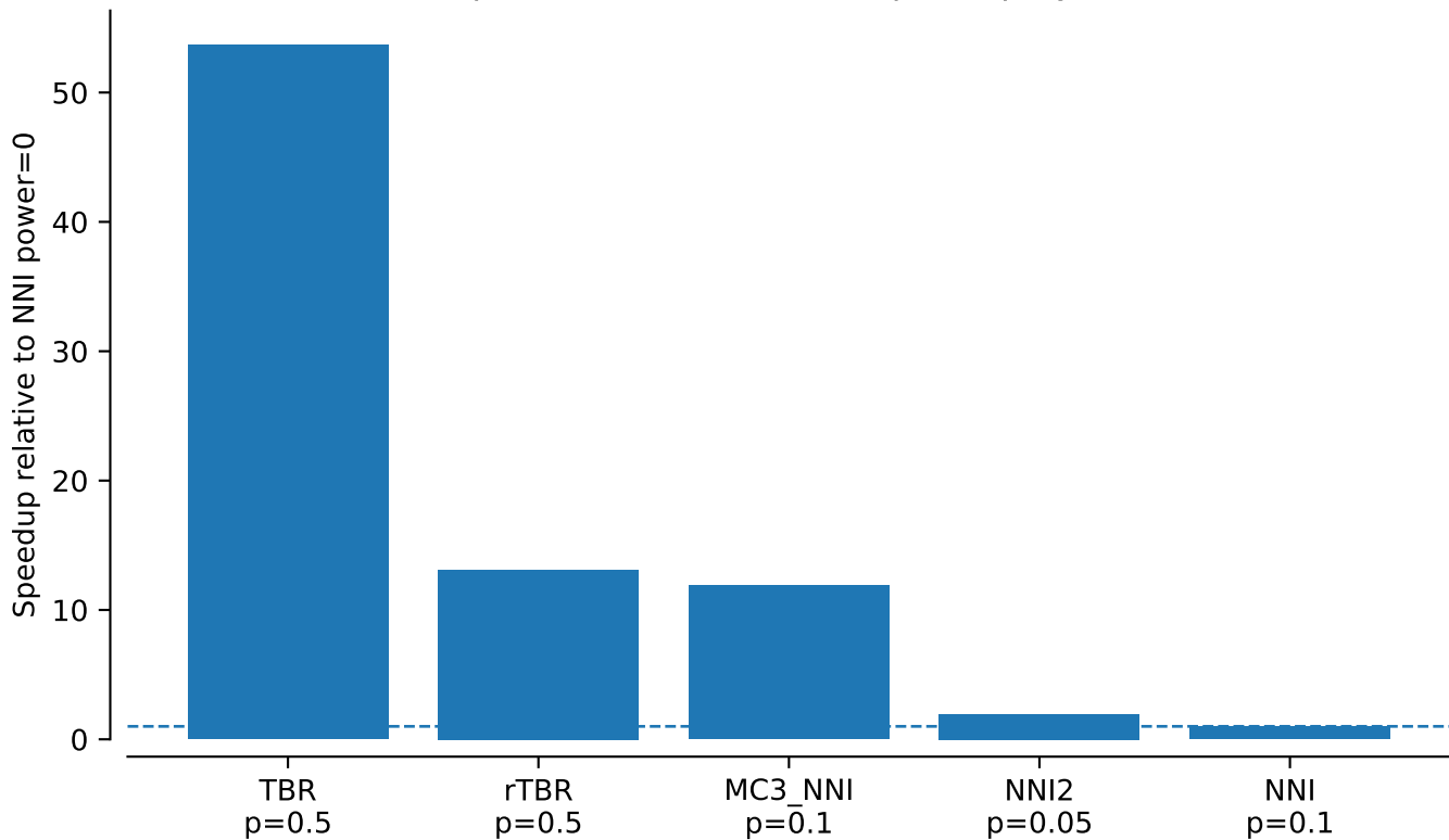
vert.atpase8.tw0: best tau95 speedup by method
