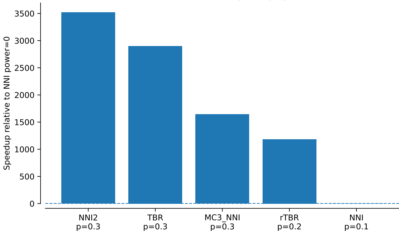
vert.coi.tw5: best tau95 speedup by method
