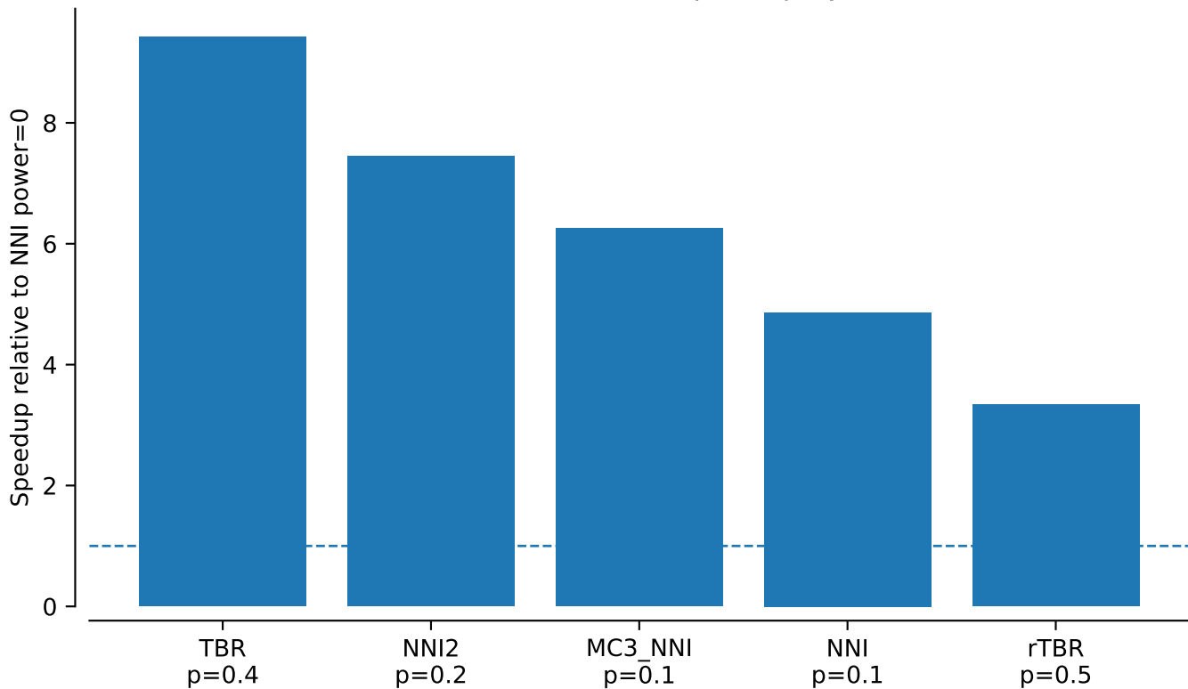
vert.nd2.tw0: best tau95 speedup by method
