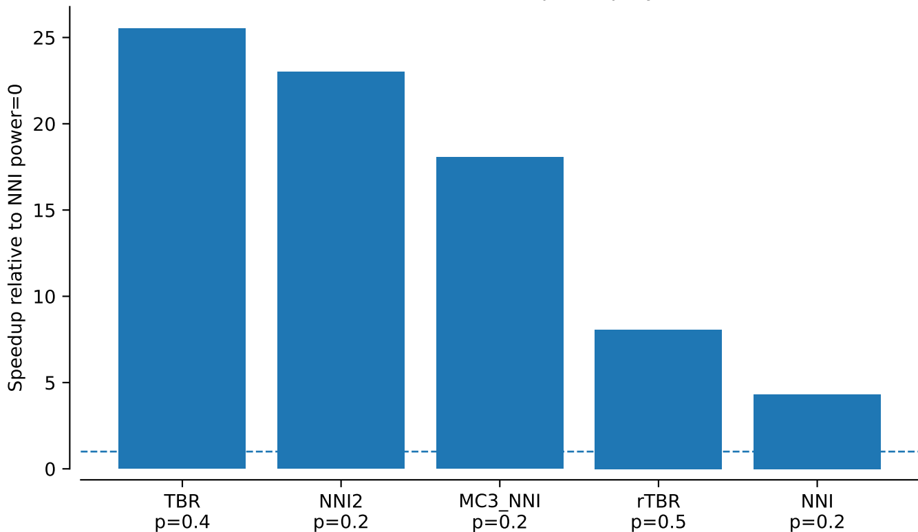
vert.nd4.tw5: best tau95 speedup by method
