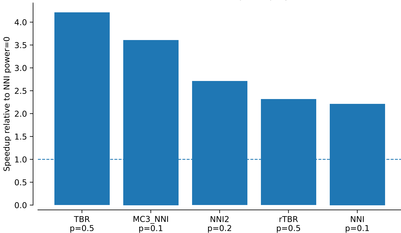
vert.nd4l.tw0: best tau95 speedup by method
