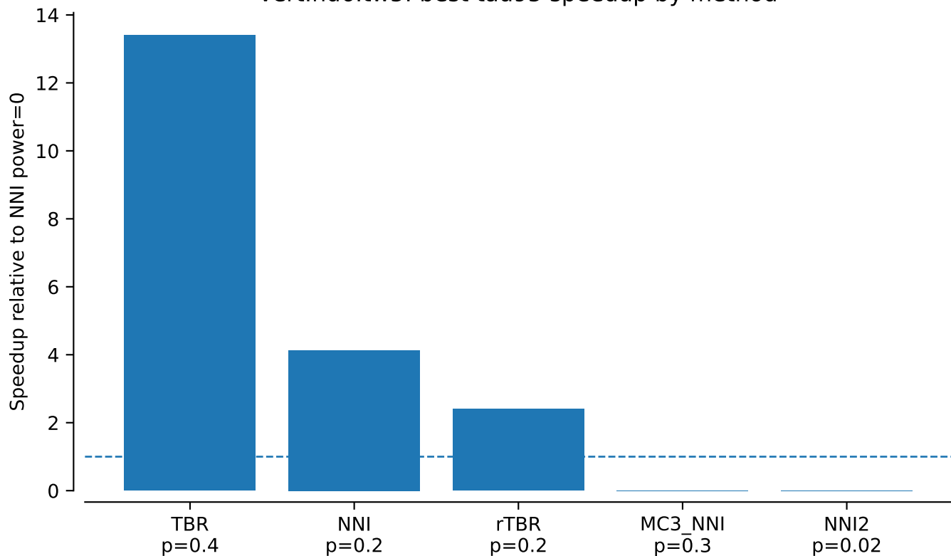
vert.nd6.tw5: best tau95 speedup by method
