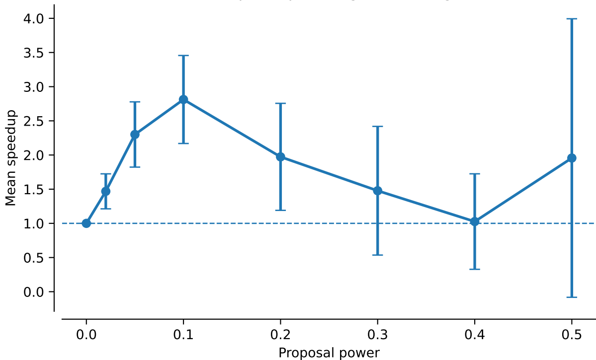
NNI tau95 speedup averaged over alignments
