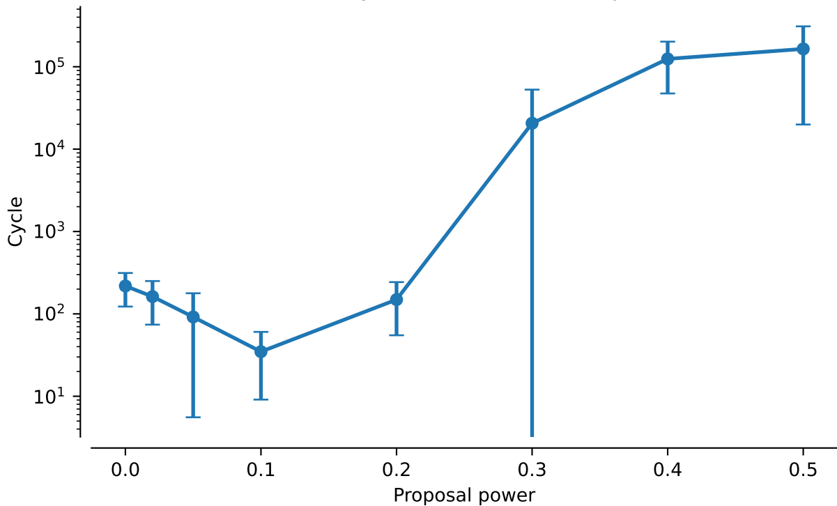
vert.coi.tw0: NNI Cycles to discover 95% posterior mass
