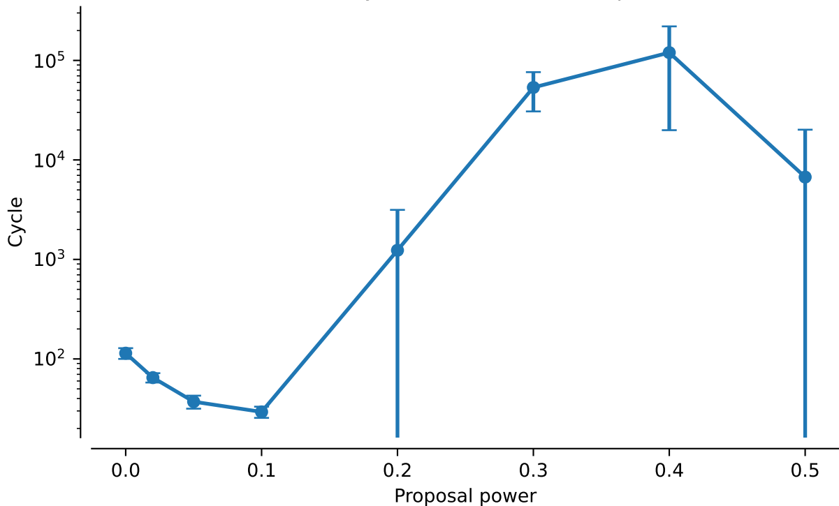
vert.coii.tw0: NNI Cycles to discover 95% posterior mass
